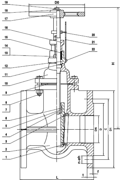
PN16 Ductile Iron Non Rising Stem Gate Valve
